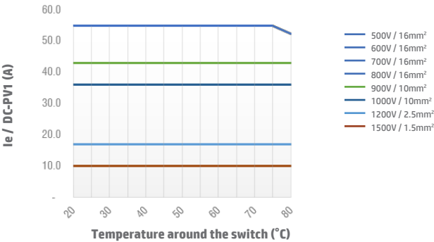
Switch SI55 2 poles DC-PV1 Enclosed Type
