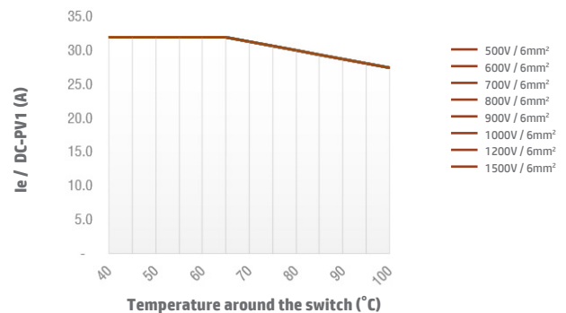
Switch SI32 4B/4S/4T DC-PV1 Open Type
