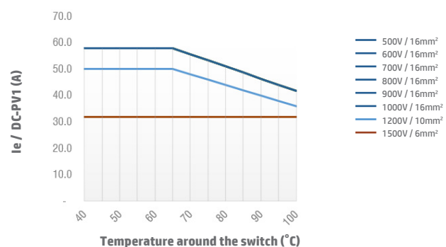
Switch SI32 4H DC-PV1 Open Type
