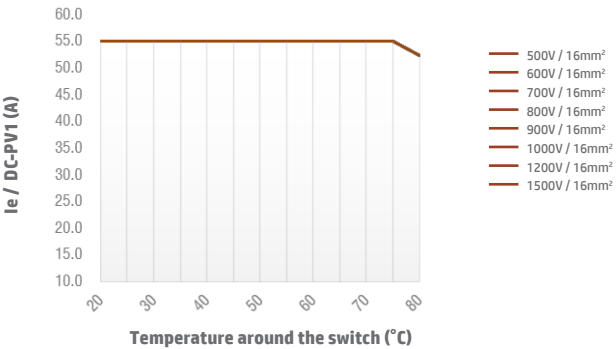
Switch SI55 4B/4S/4T DC-PV1 Enclosed Type
