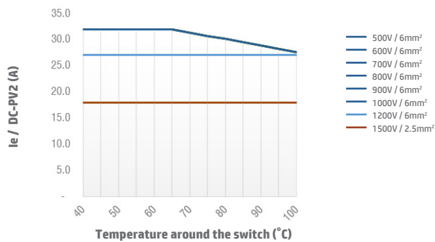
Switch SI32 4B/4S/4T DC-PV2 Open Type
