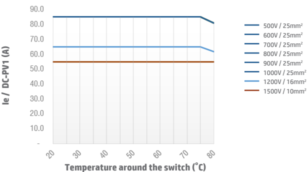
Switch SI55 4H DC-PV1 Enclosed Type
