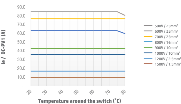
Switch SI55 2H DC-PV1 Enclosed Type
