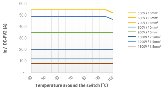
Switch SI55 2 poles DC-PV2 Open Type
